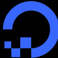
Digital Ocean
