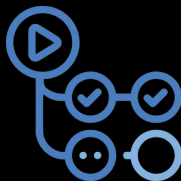
GitHub Actions
