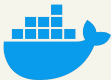
Docker
